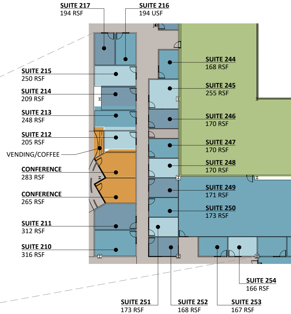
0 10 30 scale: 1" = 30'-0" ENLARGED PLAN
